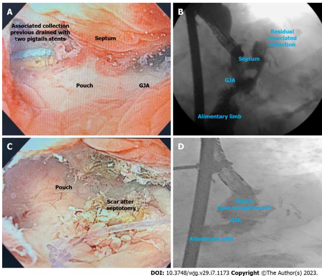
Figure 11 Septotomy. A: Septum between the associated collection and the leak orifice at the gastrojejunal anastomosis staple line after Roux-en-y gastric bypass surgery; B: Fluoroscopy showing a septum between the leak associated collection and the gastric pouch; C: Endoscopic image after septotomy; D: Fluoroscopy showing a gastric pouch without associated collections as the septotomy transformed the pouch and the associated collection in one compartment. GJA: Gastrojejunal anastomosis.
